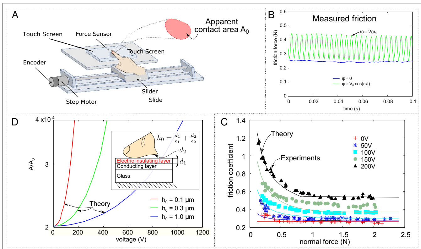
Fig. 3. Experimental and theoretical results. (A) Schematic of the experimental setup for measuring the force responses of the index finger in the normal and tangential directions, when subjected to a relative sliding motion with respect to the touchscreen. (B) Measured friction force F_f as a function of time. The green colored response was obtained by applying an oscillating electric potential to the touchscreen \phi = V_0 \cos(\omega_0 t) [where V_0 = 200 V and f_0 = \omega_0/(2\pi) = 125 Hz]. (C) The friction coefficient \mu obtained from the theory (solid lines) and the experiments (markers) as a function of the applied normal force F_N . The amplitude of the voltage applied to the touchscreen is varied between 0 V (red) and 200 V (black), with an increment of 50 V, at 125 Hz. The relative sliding speed in the experiments was 50 mm/s. In the calculations, we used E_{SC} = 40 MPa, d = 200 \mu\text{m} , E_{\text{bulk}} = 10 kPa, and h_0 = 0.2 \mu\text{m} . (D) The normalized contact area A/A_0 as a function of the applied voltage V and the thickness of the effective insulating layer h_0 = d_1/\epsilon_1 + d_2/\epsilon_2 . The applied pressure is p_0 = 10 kPa.
