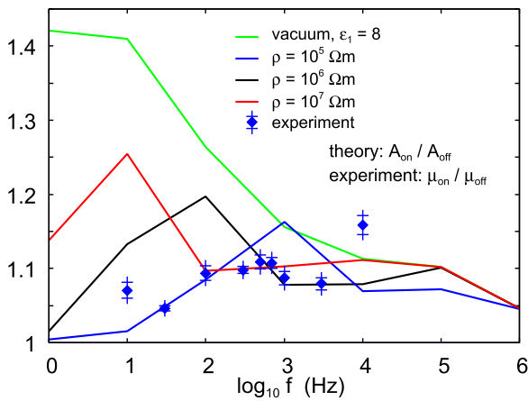
Fig. 4. (Solid lines) The calculated dependency of the contact area on the frequency f = \omega / (2\pi) of the oscillating electric potential \phi = V_0 \cos(\omega t) . The A_{on}/A_{off} is the ratio of the real contact area with electroadhesion to that without electroadhesion. The diamond symbols are the measured data for the ratio of friction coefficients with and without electroadhesion, \mu_{on}/\mu_{off} . See the first section in Discussion for details.
