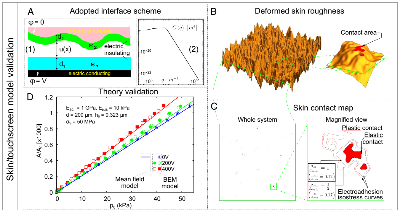
Fig. 2. Skin–touchscreen mean field model properties and validation against the predictions of BEM simulations. (A) Adopted microcontact model: an elastic solid with surface roughness above a rigid solid with a flat surface (1) and the PSD used for the comparison of the models (2). An electric voltage difference V occurs between the two conducting solids. (B) BEM-predicted roughness upon contact, with a magnified view of the surface and representation of the contact domain. The rough contact is simulated with 16 divisions at the small roughness wavelength. (C) BEM-predicted skin microcontact map, with magnified view of the map and indication of the contact domain. The black and red contour lines show the electroadhesive iso-stress curves around the true contact areas ( h_{rms} is the rms surface roughness). (D) Comparison between the normalized contact area as a function of the contact pressure, at different values of applied voltage difference across the interface.
