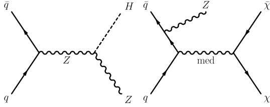
Fig. 1. Leading tree-level diagrams for the ZH production (left) and the WIMP pair production in the benchmark model (right).
