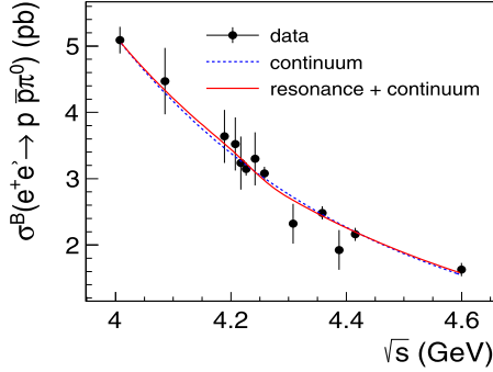
Fig. 2. Fit to \sigma(e^+e^- \rightarrow p\bar{p}\pi^0) with resonance and continuum (solid line), or only continuum term (dashed line). Dots with error bars are the measured Born cross sections. The uncertainties are statistical only.
