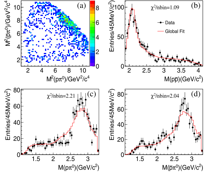
Fig. 1. (a) Dalitz plot for the selected e^+e^- \rightarrow p\bar{p}\pi^0 candidates of data and invariant mass spectra of (b) p\bar{p} , (c) p\pi^0 and (d) \bar{p}\pi^0 at \sqrt{s} = 4.258 \text{ GeV} . In (b), (c) and (d), the points with error bars show data and the red histograms show MC projections of the partial wave analysis fit described in the text. (For interpretation of the references to color in this figure legend, the reader is referred to the web version of this article.)
