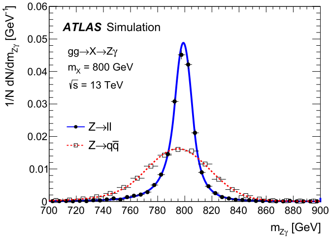
Fig. 1. Invariant-mass distribution for X \rightarrow Z\gamma , Z \rightarrow \ell\ell (solid circles) or Z \rightarrow q\bar{q} events (open squares) in a simulation of a narrow resonance X with a mass of 800 GeV produced in a gluon-fusion process in \sqrt{s} = 13 TeV pp collisions. All selection requirements have been applied. The blue solid (red dashed) line represents the fit of the points with a double-sided Crystal Ball function (sum of a Crystal Ball function and a Gaussian function).
