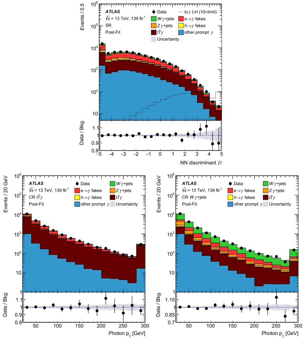
Fig. 4. Post-fit distributions of a background-only fit to the NN discriminant in the SR for the tu\gamma coupling (top) and the photon p_T distribution in the t\bar{t}\gamma (bottom left) and W\gamma +jet CRs (bottom right). The last bin of the distributions contains the overflow and in the case of the SR, the first bin also contains the underflow. In addition, in the SR, the expected tu\gamma LH signal is overlaid for an expected number of events corresponding to the observed 95% CL limit scaled by a factor of ten, representing BR for the t \rightarrow u\gamma LH coupling of 8.5 \times 10^{-5} . The lower panels show the ratios of the data ('Data') to the background prediction ('Bkg.'). The uncertainty band includes both the statistical and systematic uncertainties in the background prediction. Correlations among uncertainties were taken into account as determined in the fit.
