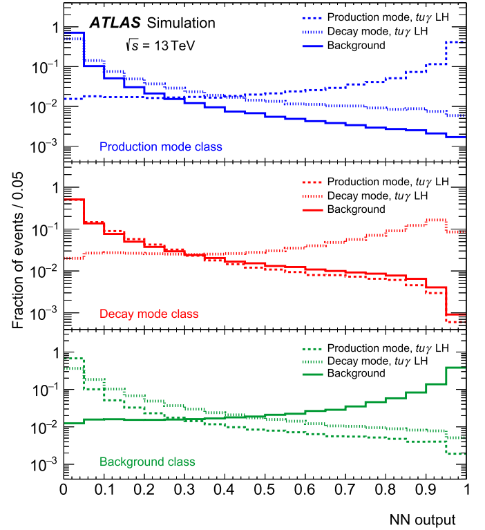
Fig. 3. The classifier output of the multiclass NN for the tu\gamma LH coupling. The output of the FCNC production mode class is shown in blue (top), the output of the FCNC decay mode class is shown in red (middle) and the output of the SM background class is shown in green (bottom). For each output class, the distribution of the three processes is shown: FCNC production mode with the dashed line, FCNC decay mode with the dotted line and SM background with the solid line. The vertical axis represents the fraction of events predicted by the simulation.
