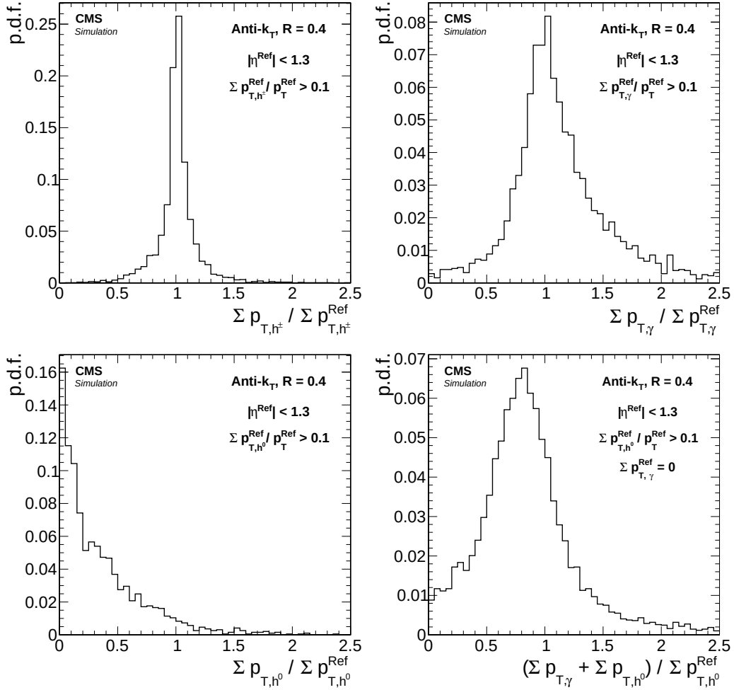
Figure 11. Distribution of the ratio between the reconstructed and reference transverse momenta, \Sigma p_{T,i} / \Sigma p_{T,i}^{\text{Ref}} , for charged hadrons (top left), photons (top right), neutral hadrons (bottom left), and for all neutral particles in Ref jets with no photon (bottom right). The Ref jet is required to have at least 10% of its p_T carried by particles of type i , and to be located in the barrel.
