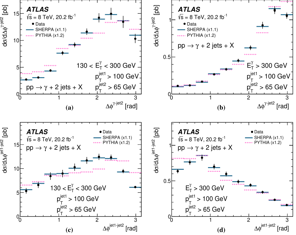
Fig. 11. Measured cross sections for isolated-photon plus two-jet production (dots) as functions of (a, b) \Delta\phi^{\gamma\text{--jet}2} and (c, d) \Delta\phi^{\text{jet}1\text{--jet}2} for (a, c) E_T^\gamma < 300 GeV and (b, d) E_T^\gamma > 300 GeV. For comparison, the predictions from PYTHIA (dashed lines) and SHERPA (solid lines) are also shown. The predictions are normalised to the data by a global factor, which is indicated in parentheses. The inner (outer) error bars represent the statistical uncertainties (the statistical and systematic uncertainties added in quadrature). For most of the points, the inner error bars are smaller than the marker size and, thus, not visible.
