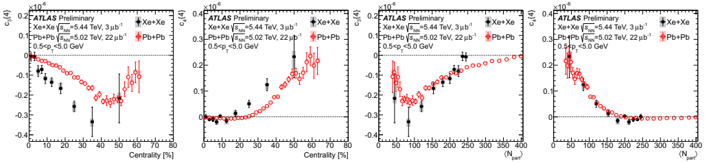
Fig. 3. The 4-particle cumulant, c_4\{4\} as a function centrality (two left panels) and number of collision participants, N_{\text{part}} , (two right panels) in Xe+Xe data at 5.44 TeV compared to Pb+Pb at 5.02 TeV [3].
