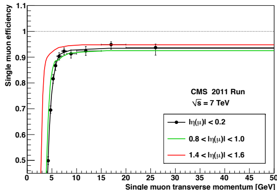
Figure 69. Single-muon detection efficiencies (convolving trigger, reconstruction, and selection requirements) as a function of p_T , as obtained from the data, using the tag-and-probe method. Data points are shown for the pseudorapidity range |\eta| < 0.2 , while the curves (depicting a parametrization of the measured efficiencies) correspond to the three ranges indicated in the legend.
