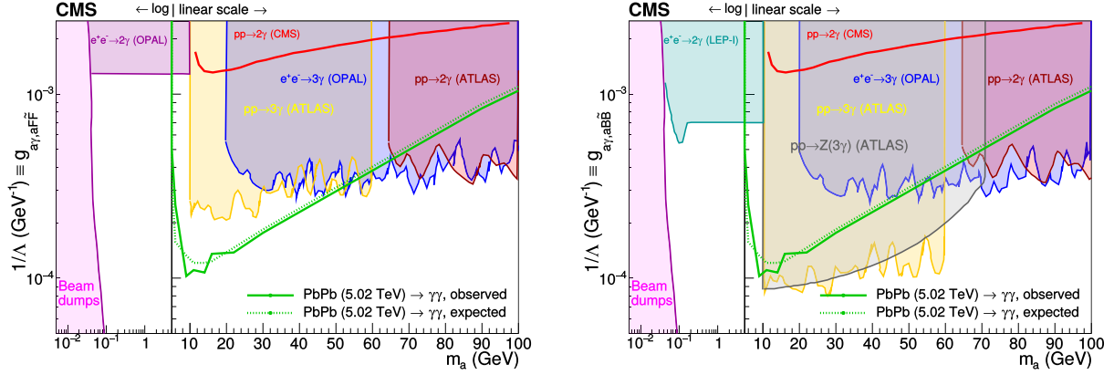
Fig. 7. Exclusion limits at 95% CL in the ALP-photon coupling g_{\gamma\gamma} versus ALP mass m_a plane, for the operators a\tilde{F}\tilde{F}/4\Lambda (left, assuming ALP coupling to photons only) and aB\tilde{B}/(4\Lambda\cos^2\theta_W) (right, including also the hypercharge coupling, thus processes involving the Z boson) derived in Refs. [30,56] from measurements at beam dumps [60], in e^+e^- collisions at LEP-I [56] and LEP-II [57], and in pp collisions at the LHC [13,58,59], and compared to the present PbPb limits.
