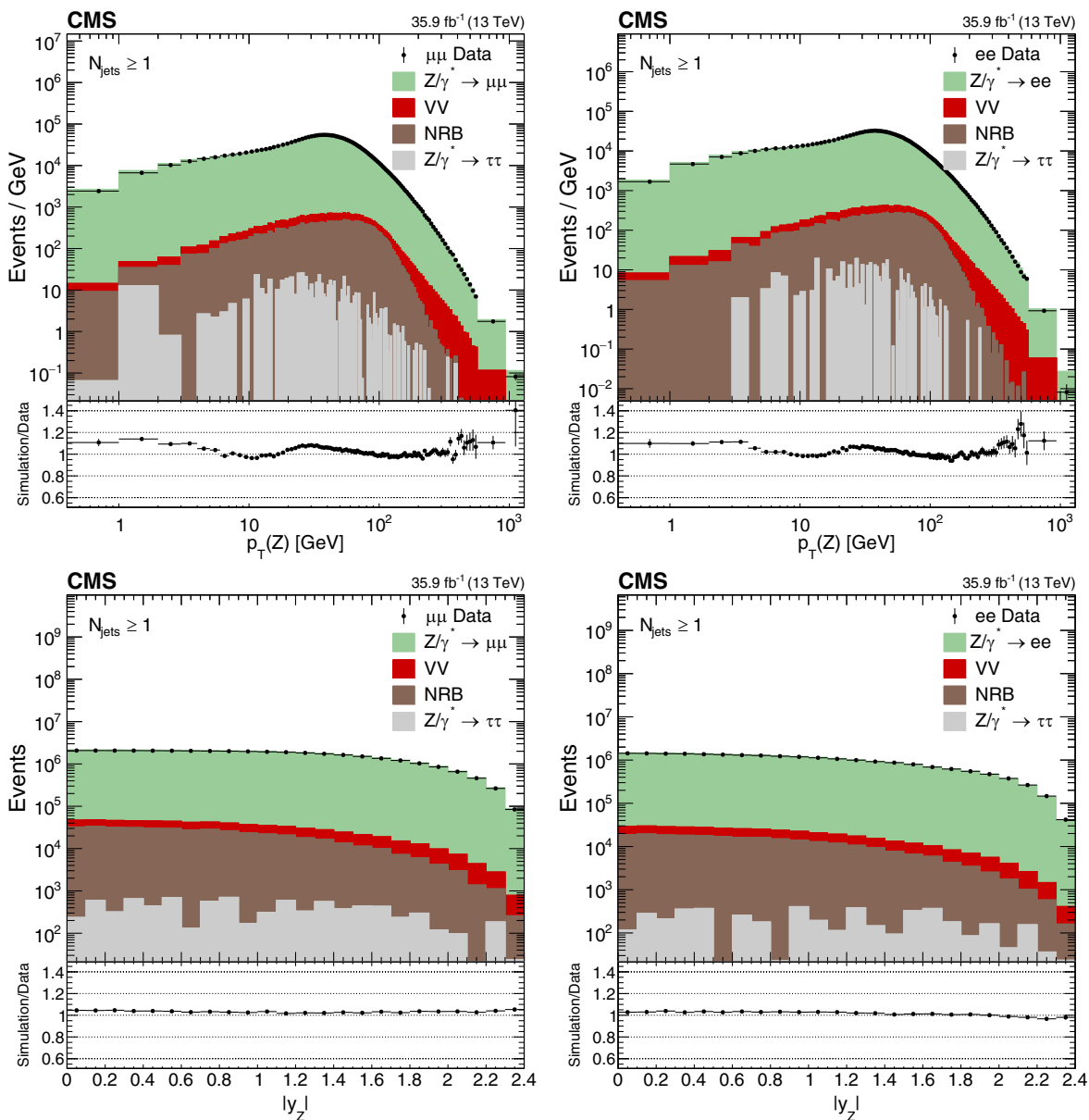
FIG. 1. The Z boson candidate p_T (upper) and |y| (lower) for events with at least one jet. The muon (left) and electron (right) channels are shown separately. The background is estimated from both simulation and data driven methods (such as nonresonant background, NRB) as described in Sec. VII. The error bars around the data points represent the statistical uncertainties. The distribution ratio of simulation to data is shown in the bottom frames, with error bars that represent the total statistical uncertainties from the data and simulation samples.
