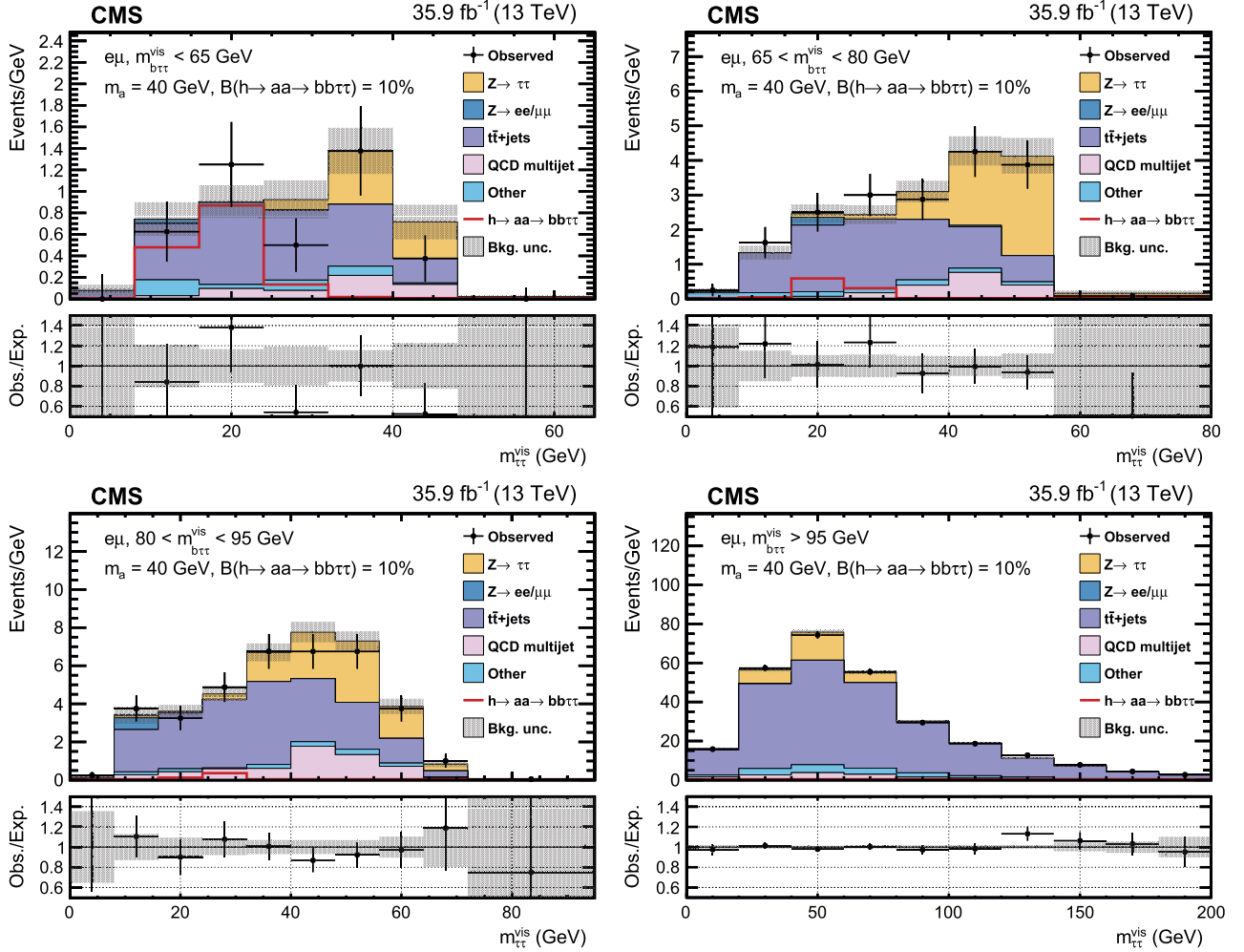
Fig. 4. Distributions of m_{\tau\tau}^{vis} in the four categories of the e\mu channel. The “Other” contribution includes events from single top quark, diboson, SM Higgs boson, and W + jets productions. The signal histogram corresponds to the SM production cross section for ggh , VBF , and Vh processes, and assumes \mathcal{B}(h \rightarrow aa \rightarrow 2\tau 2b) = 10\% . The normalizations of the predicted background distributions correspond to the result of the global fit.
