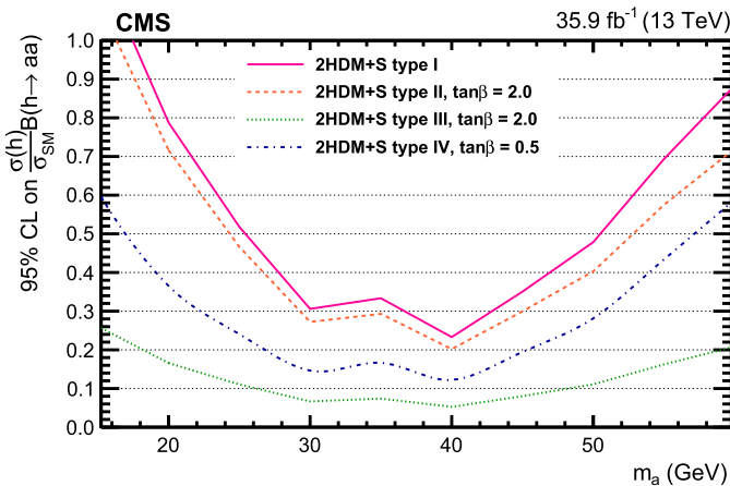
Fig. 9. Observed 95% CL limits on (\sigma(h)/\sigma_{\text{SM}})B(h \rightarrow aa) for various 2HDM + S types. The limit in type I 2HDM + S does not depend on \tan \beta .
