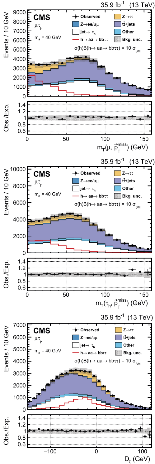
Fig. 3. Distributions of m_T(\mu, \vec{p}_T^{\text{miss}}) (top), m_T(\tau_h, \vec{p}_T^{\text{miss}}) (center), and D_\xi (bottom) in the \mu\tau_h final state before the m_T^{\text{vis}} -based categorization. The “jet \rightarrow \tau_h ” contribution includes all events with a jet misidentified as a \tau_h candidate, whereas the rest of background contributions only include events where the reconstructed \tau_h corresponds to a \tau_h , a muon, or an electron, at the generator level. The “Other” contribution includes events from single top quark, diboson, and SM Higgs boson processes. The signal histogram corresponds to 10 times the SM production cross section for ggh, VBF, and Vh processes, and assumes \mathcal{B}(h \rightarrow aa \rightarrow 2\tau 2b) = 100\% .
