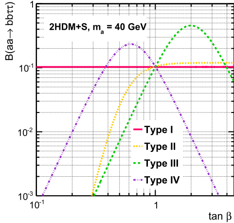
Fig. 1. Predicted B(aa \rightarrow bb\tau\tau) for m_a = 40 GeV in the different models of 2HDM + S, as a function of \tan\beta . The picture is essentially the same for all m_a hypotheses considered in this Letter. The branching fractions are computed following the formulas of Ref. [15].
