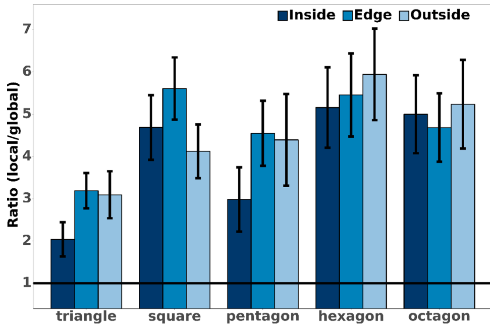
Fig. 10. The ratio of local scanning time to the global scanning time with standard error of the means for all five shapes under three rendering conditions. The horizontal solid line shows the boundary when the ratio is equal to one.
