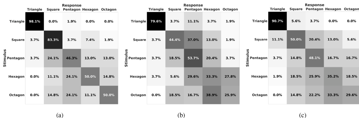
Fig. 13. Confusion metrics of the recognition rate for (a) prototypical shapes and non-prototypical shapes; (b) positive and (c) negative.
