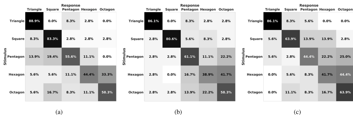
Fig. 7. Confusion metrics of the recognition rate for (a) inside, (b) edge, and (c) outside rendering conditions.
