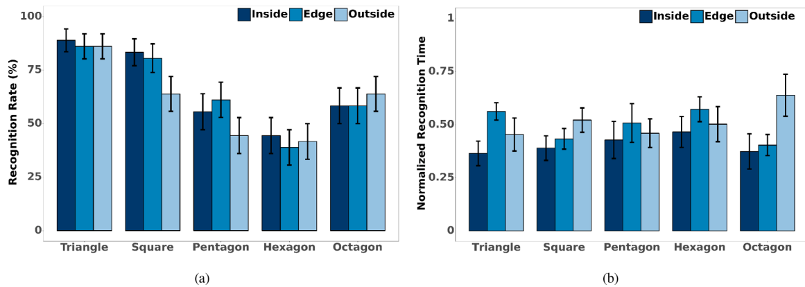
Fig. 6. (a) Recognition rate and (b) normalized recognition time with standard error of the means for all shapes and rendering conditions.
