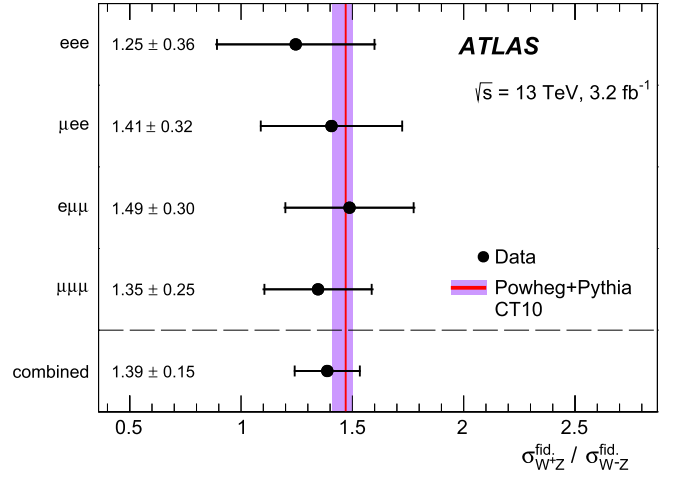
Fig. 3. Measured ratios \sigma^{\text{fid.}}_{W^\pm Z} / \sigma^{\text{fid.}}_{W^\pm Z} of W^+ Z and W^- Z integrated cross sections in the fiducial phase space in each of the four channels and for their combination. The error bars on the data points represent the total uncertainties, which are dominated by the statistical uncertainties. The NLO SM prediction from POWHEG+PYTHIA using the CT10 PDF set is represented by the red line; the shaded violet band is the total uncertainty in this prediction. (For interpretation of the references to colour in this figure legend, the reader is referred to the web version of this article.)
