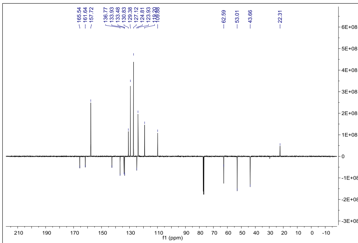
Figure S6. APT spectrum of Compound 4a.
