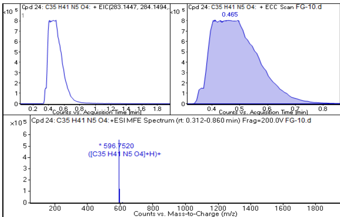
Figure S43. HRMS Spectrum of Compound 10.
