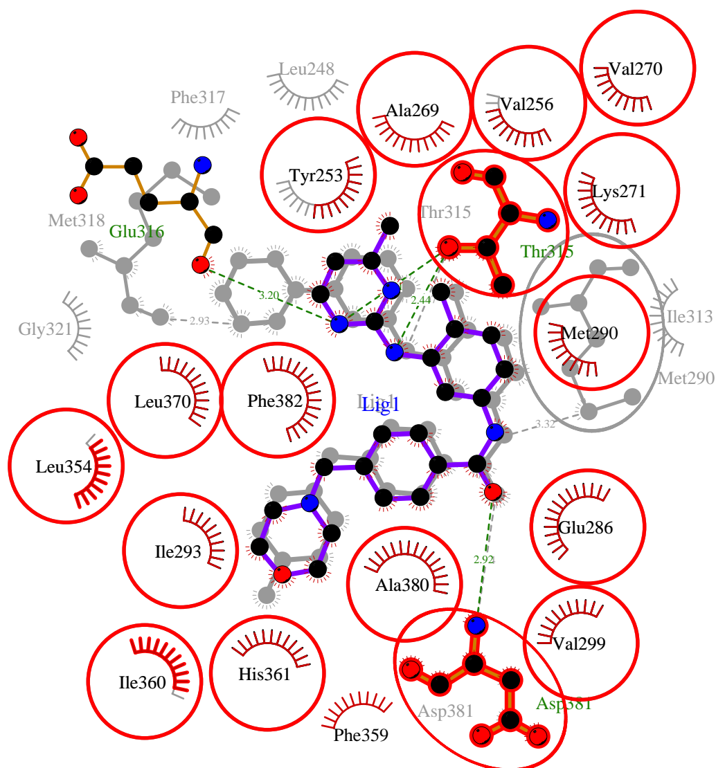
Figure S48. Comparison of ABL-imatinib (background) and ABL-Compound 8 (foreground) interactions. Imatinib and its contact residues are depicted in gray, while the common contact residues are marked with red circles.
