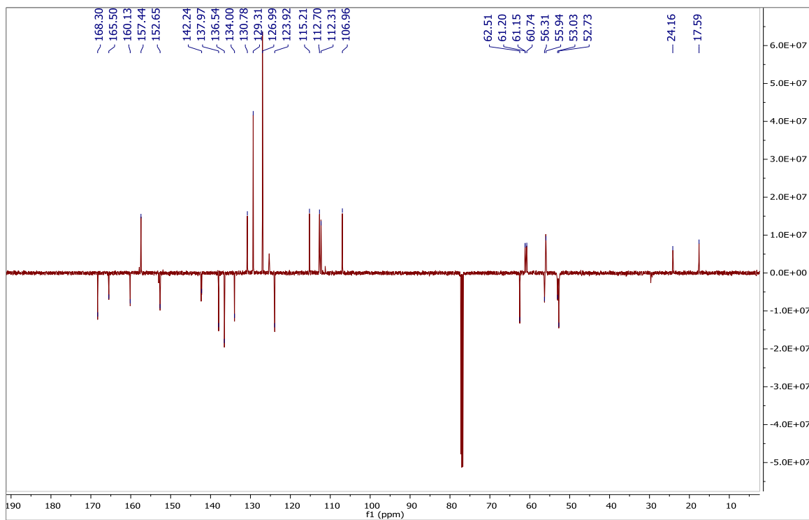
Figure S26. APT spectrum of Compound 6.
