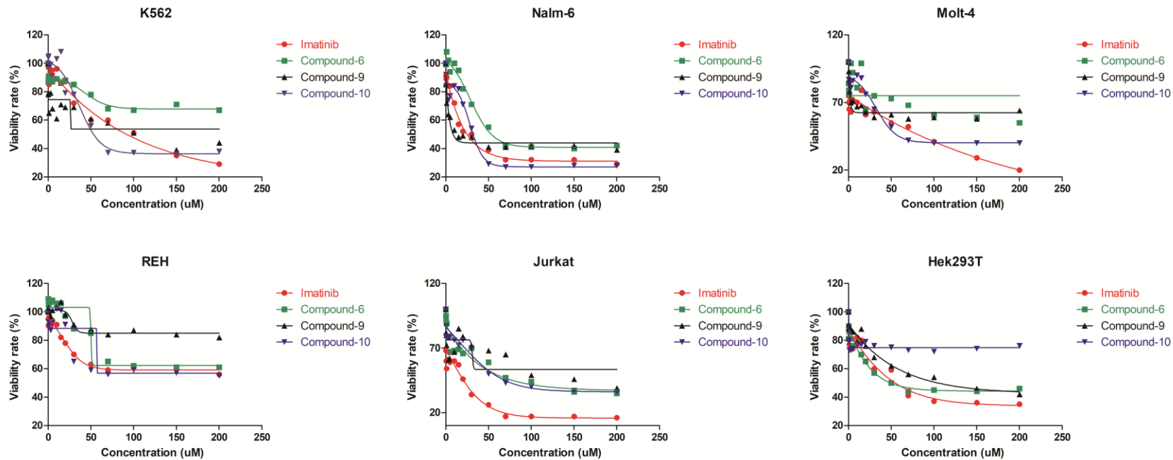
Figure S44. Comparison between imatinib and compound-6-9-10 in all cell-lines.
