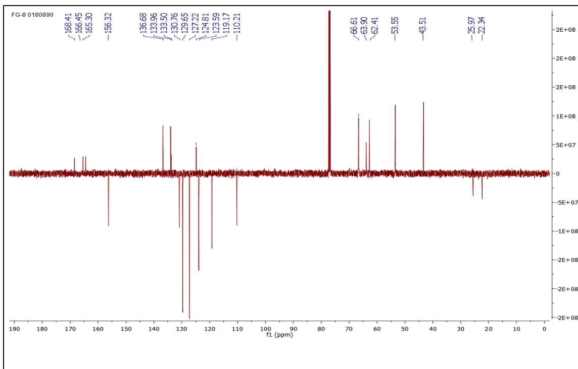
Figure S34. APT spectrum of Compound 8.
