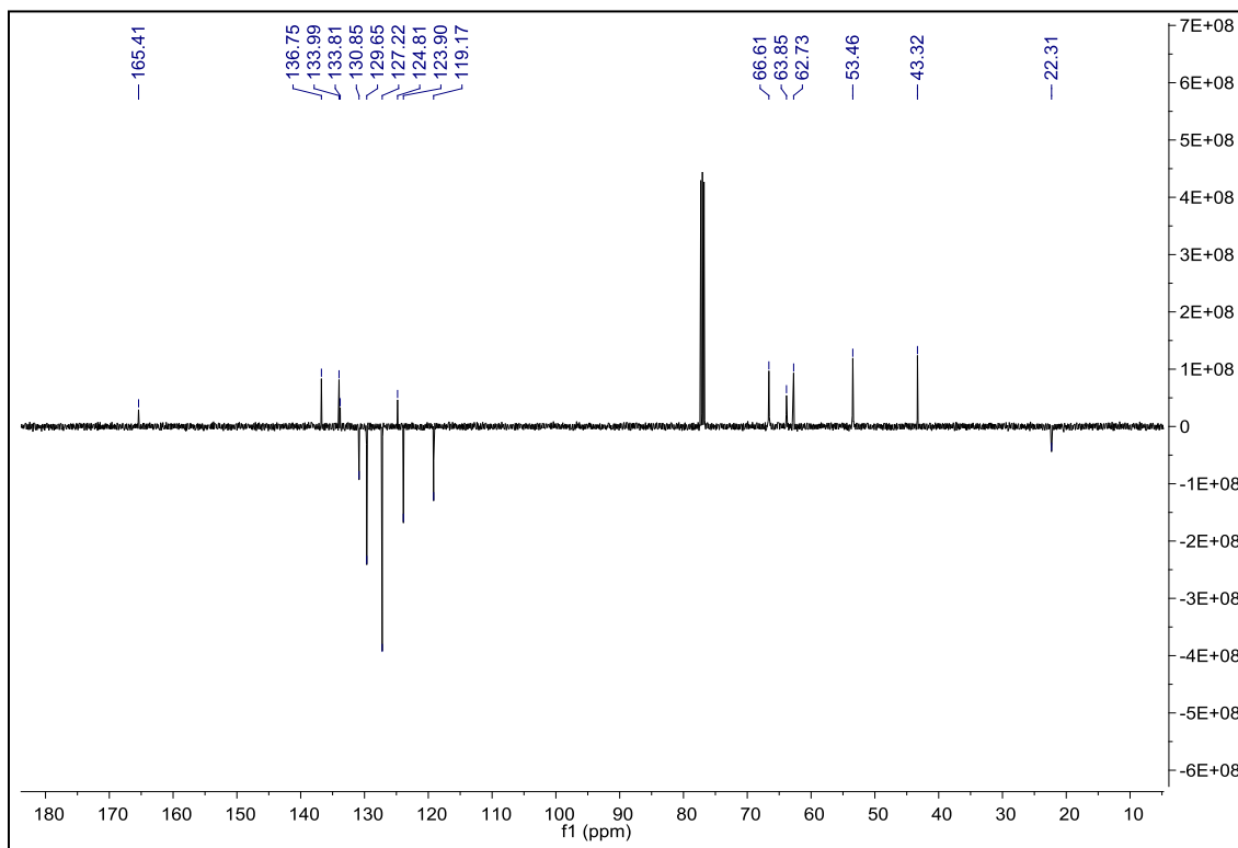
Figure S16. APT spectrum of Compound 4c.
