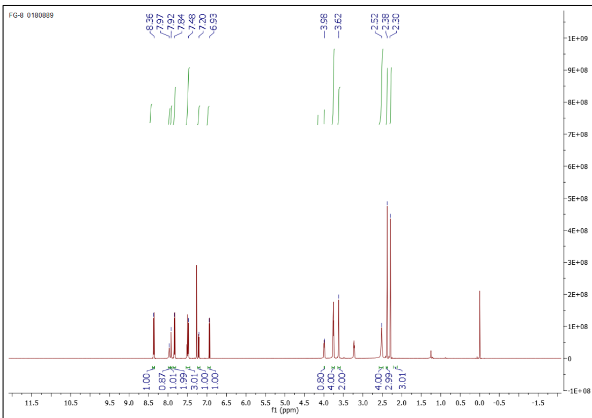
Figure S33. ^1\text{H-NMR} spectrum of Compound 8.
