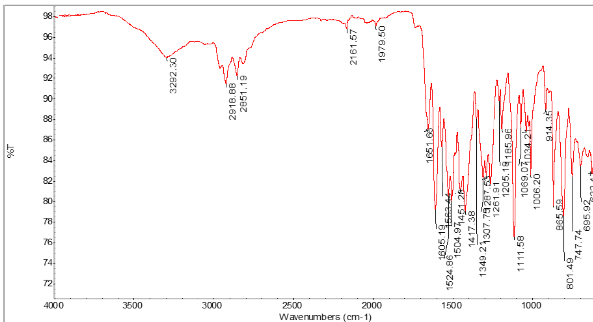
Figure S36. IR spectrum of Compound 9.
