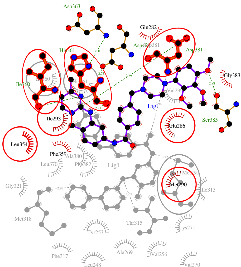
Figure S46. Comparison of ABL-imatinib (background) and ABL-Compound 6 (foreground) interactions. Imatinib and its contact residues are depicted in gray, while the common contact residues are marked with red circles.
