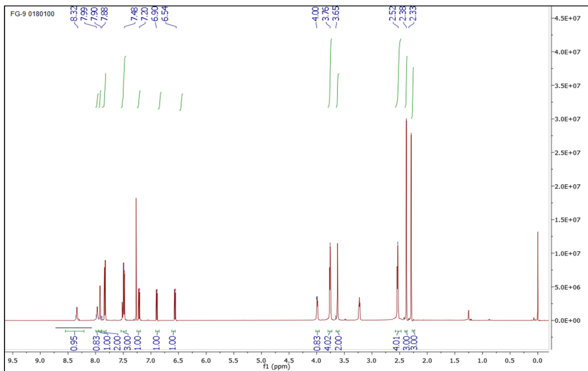
Figure S37. 1 H-NMR spectrum of Compound 9.
