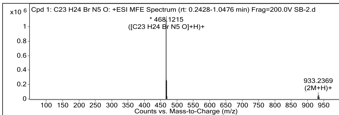
Figure S7. HRMS Spectrum of Compound 4a.
