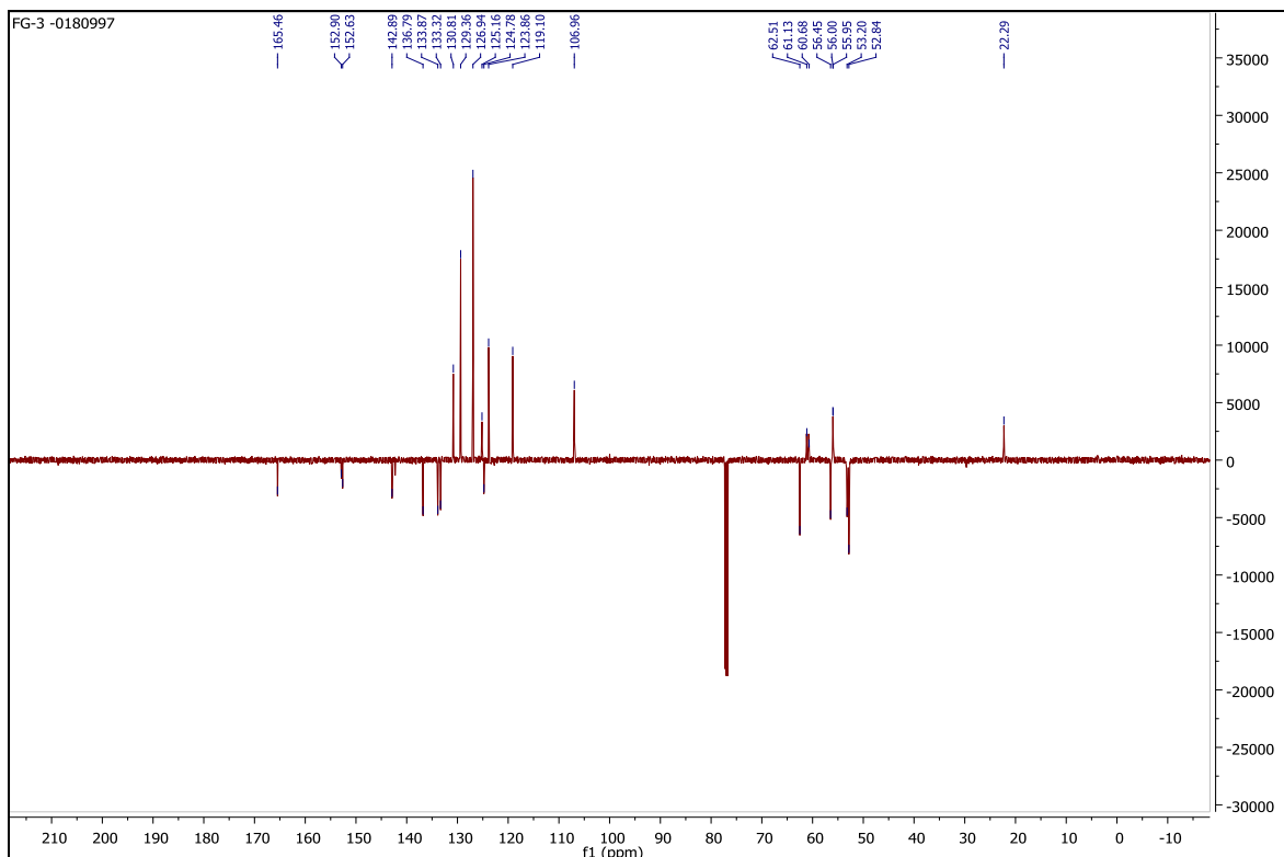
Figure S12. APT spectrum of Compound 4b.
