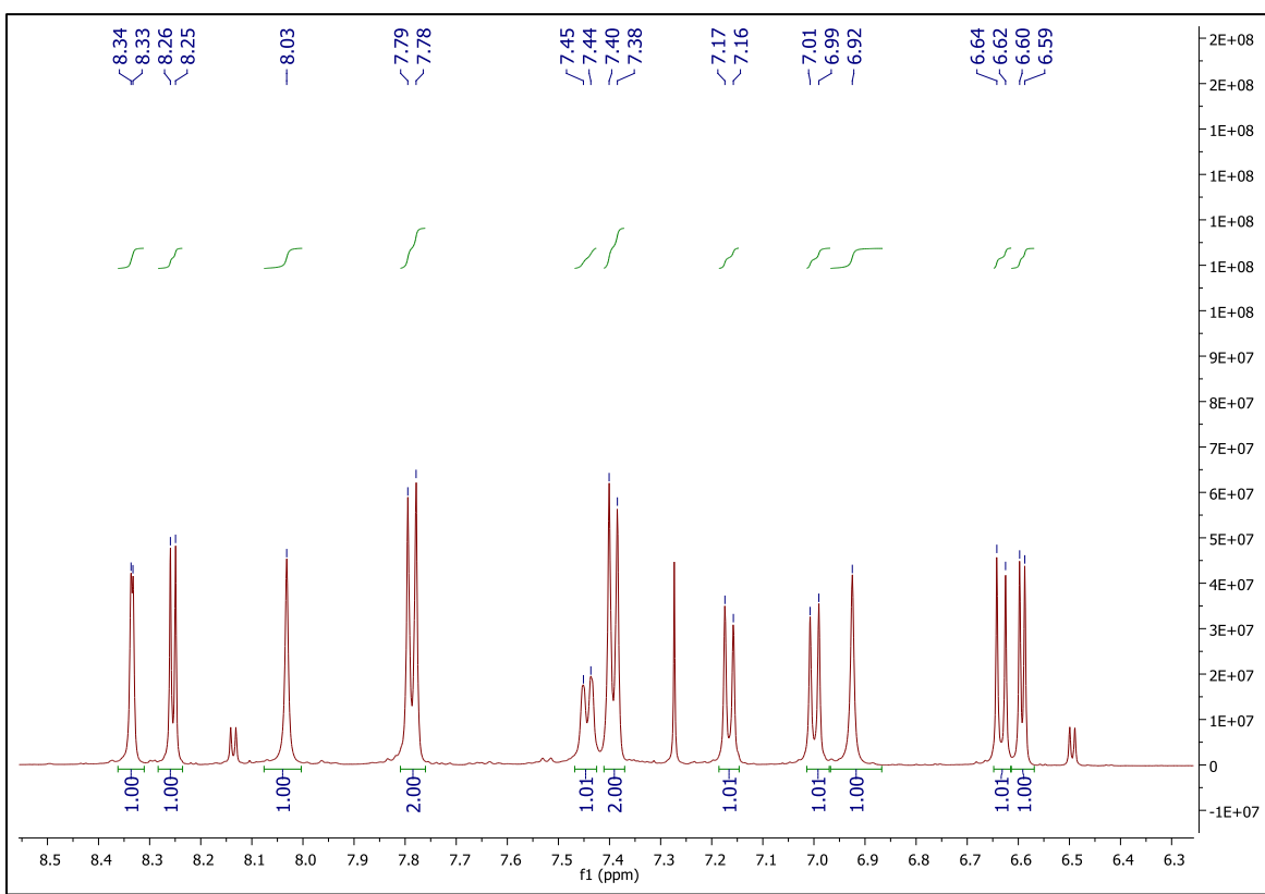
Figure S23-S24-S25. 1 H-NMR spectrum of Compound 6.
