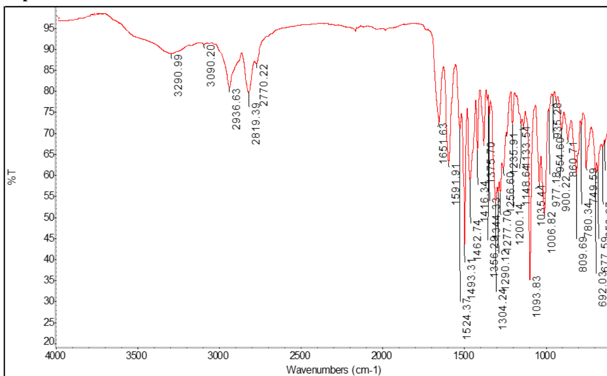
Figure S8. IR spectrum of Compound 4b.
