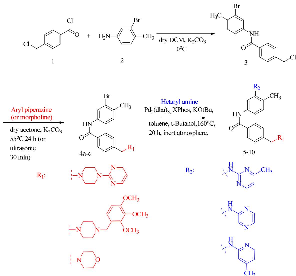
Scheme. Synthesis route of novel imatinib derivatives (compound 5-10).
