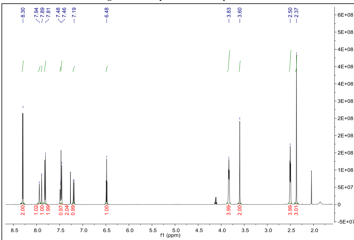
Figure S5. ^1\text{H-NMR} spectrum of Compound 4a.
