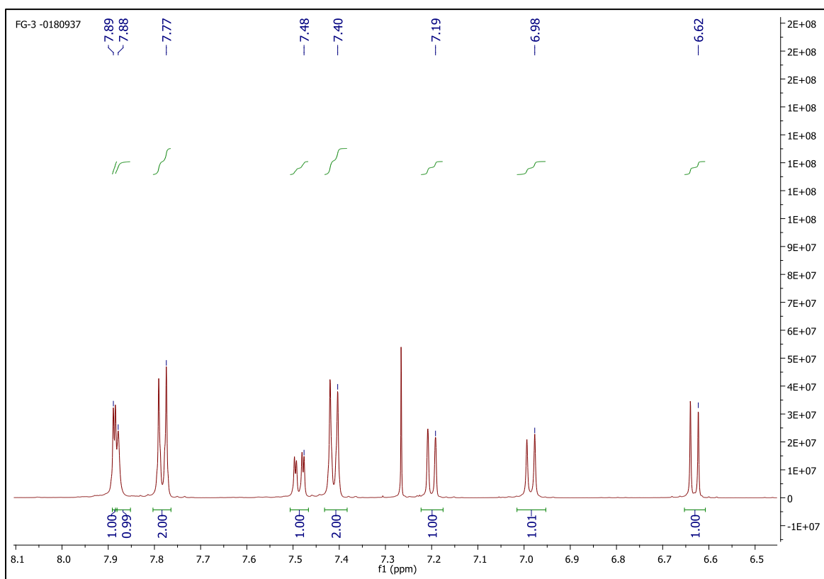
Figure S10-S11. ^1\text{H-NMR} spectrum of Compound 4b.
