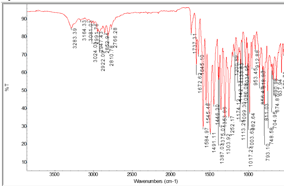
Figure S4. IR spectrum of Compound 4a.
