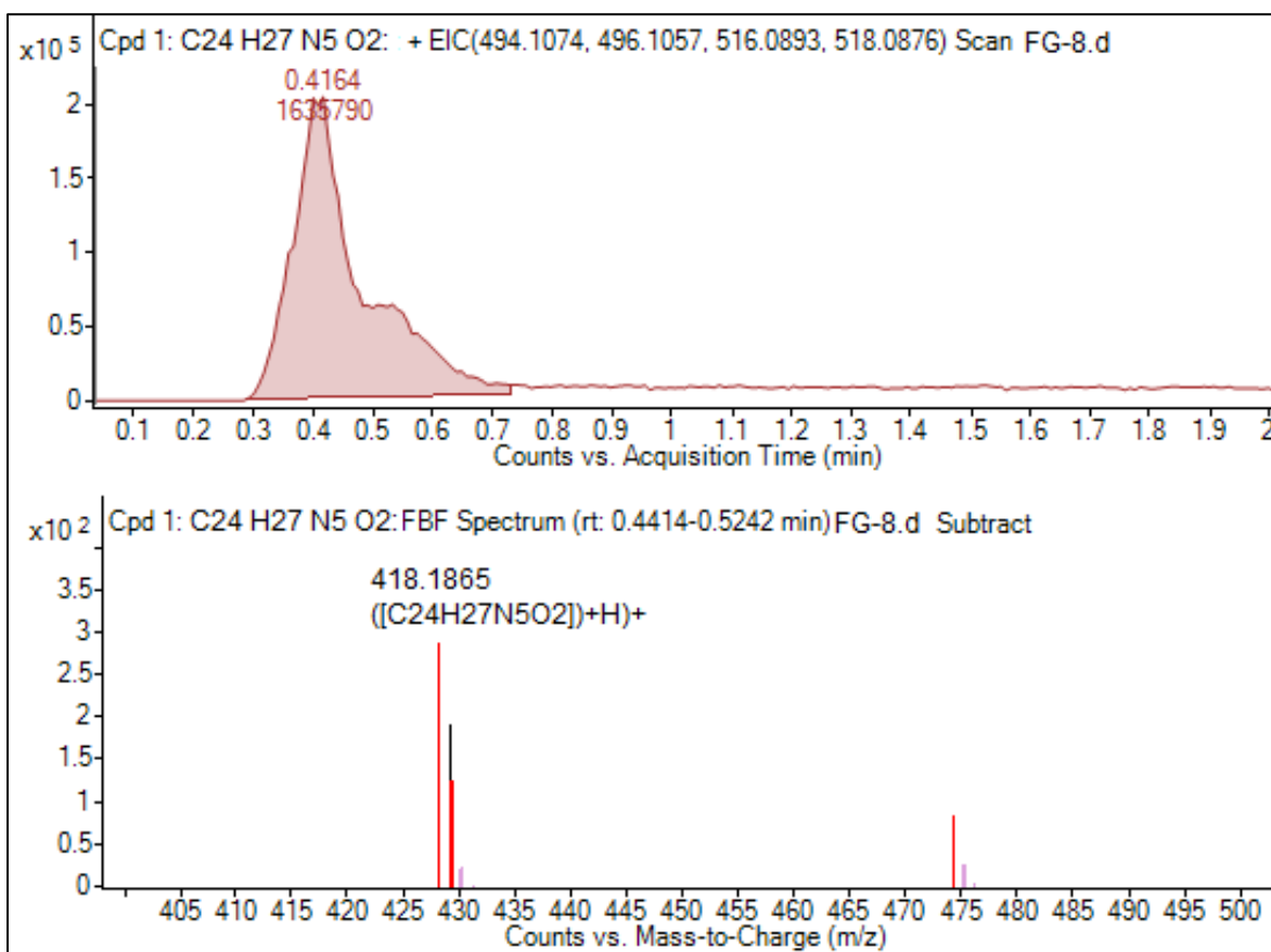
Figure S35. HRMS Spectrum of Compound 8.
