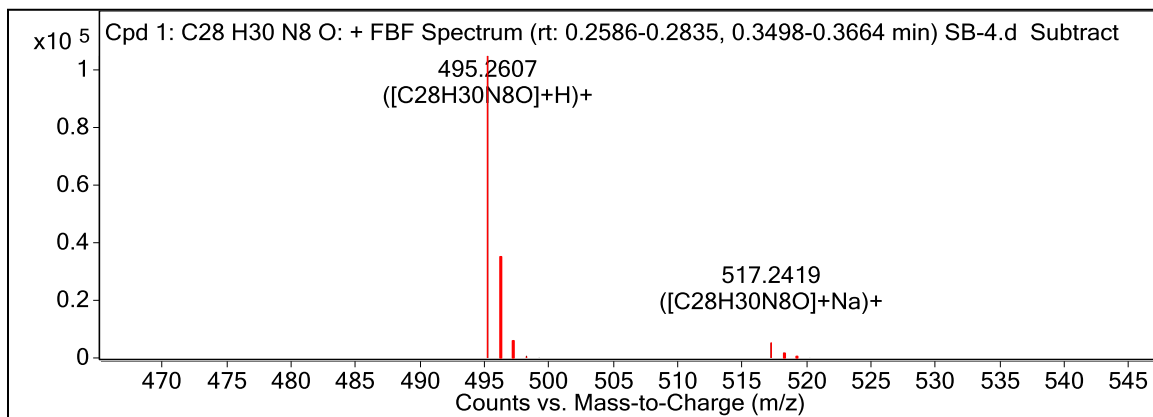
Figure S21. HRMS Spectrum of Compound 5.
