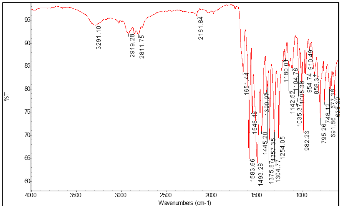
Figure S28. IR spectrum of Compound 7.
