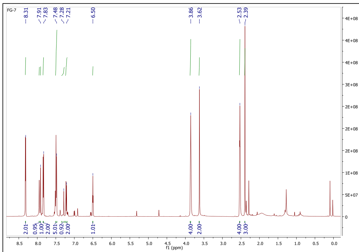
Figure S29. 1 H-NMR spectrum of Compound 7.
