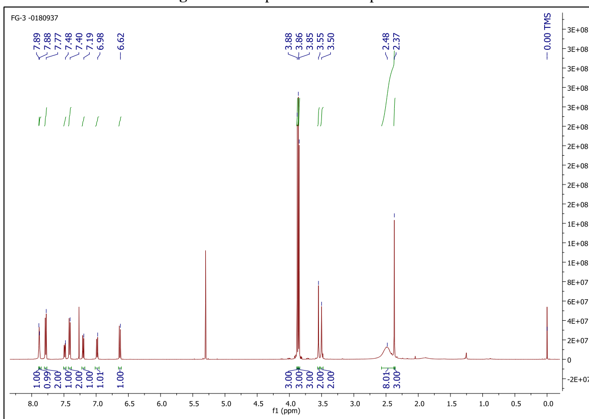
Figure S9. 1 H-NMR spectrum of Compound 4b.
