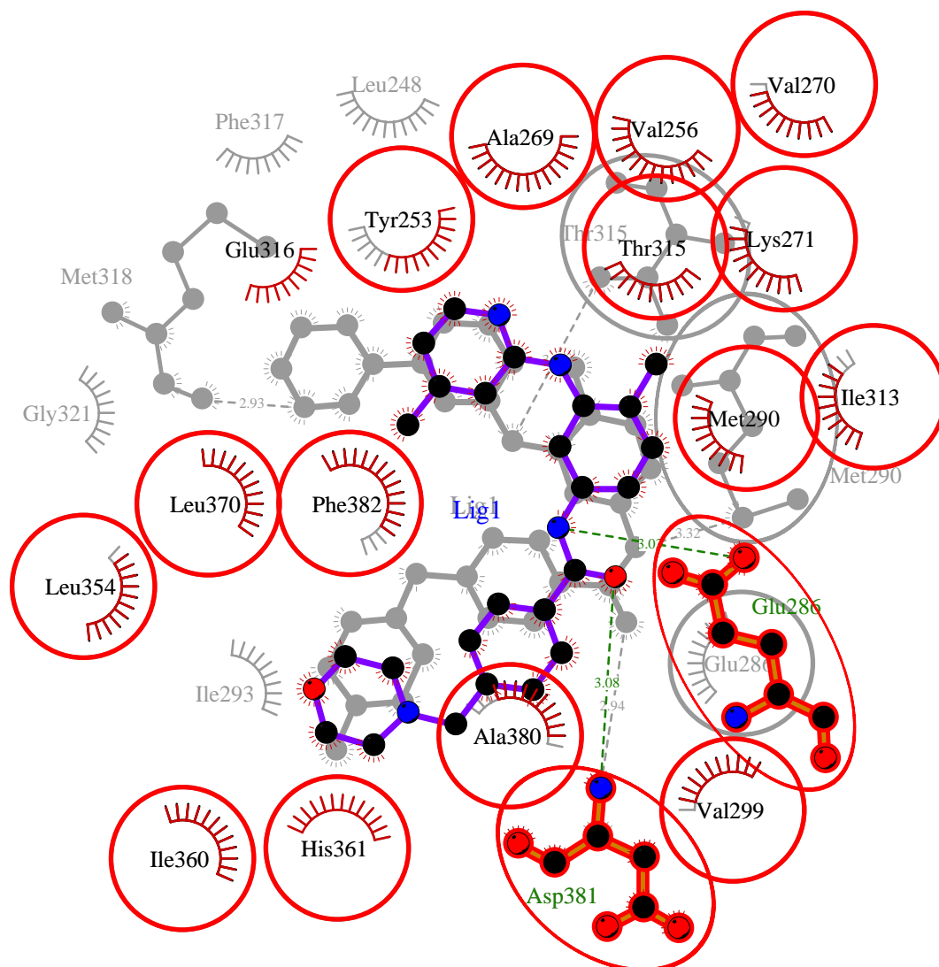
Figure S49. Comparison of ABL-imatinib (background) and ABL-Compound 9 (foreground) interactions. Imatinib and its contact residues are depicted in gray, while the common contact residues are marked with red circles.
