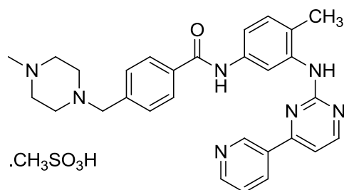
Figure 1. Imatinib mesylate molecular structure.
