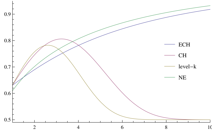
Figure 6.2.1.. The probability of correct group decision under different models. In CH, ECH and level- k models \sigma = 2 , q = 3/4 , \tau = 3 and b_0 = -1 are taken, while for NE only \sigma = 2 and q = 3/4 are relevant.
