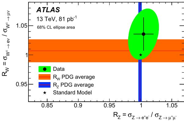
Fig. 3. Ratio of the electron- and muon-channel W^\pm and Z -boson production fiducial cross sections, compared to the expected values of the Standard Model of (1, 1) (neglecting mass effects that contribute at a level below 10^{-5} ) and previous experimental verifications of lepton universality for on-shell W^\pm and Z bosons, shown as PDG average bands [49,50]. The PDG average values and the result are shown with total uncertainties.
