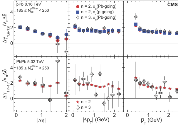
Fig. 1. The ratio of \Delta\gamma_{12} and \Delta\gamma_{123} to the product of v_n and \delta , as functions of |\Delta\eta| (left), |\Delta p_T| (middle), and \bar{p}_T (right) for 185 \leq N_{\text{trk}}^{\text{offline}} < 250 in pPb collisions at \sqrt{s_{\text{NN}}} = 8.16 TeV (upper) and PbPb collisions at 5.02 TeV (lower) [16]. Statistical and systematic uncertainties are indicated by the error bars and shaded regions, respectively.
