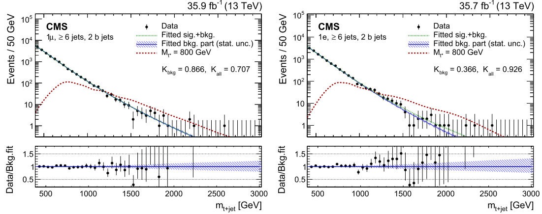
Fig. 2. The m_{t+jet} spectrum for data (points), the signal + background fit (green), the background component of the signal + background fit (blue), and the expected spectrum for a simulated 800 GeV signal process (red dashed) normalized to the integrated luminosity of data. Since there is no significant excess of signal found in data, the signal + background curve overlaps the background-only component. The distributions for the \mu + jets data are shown on the left while those for e + jets data are shown on the right. The probabilities of the Kolmogorov-Smirnov test between the data versus the signal + background model and between the data versus the background component are denoted by K_{all} and K_{bkg} , respectively. (For interpretation of the references to color in this figure legend, the reader is referred to the web version of this article.)
