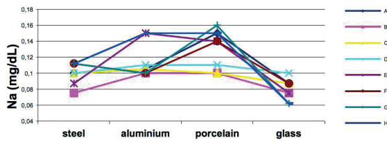
1E. Na contents of eight infusion samples in four different pots
