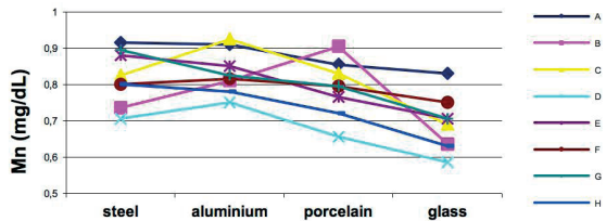
1C. Mn contents of eight infusion samples in four different pots
